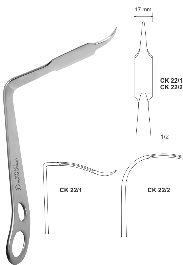
HOHMANN 240 mm (9 1/2")
