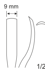
CK 10B 272 mm (10 3/4")
